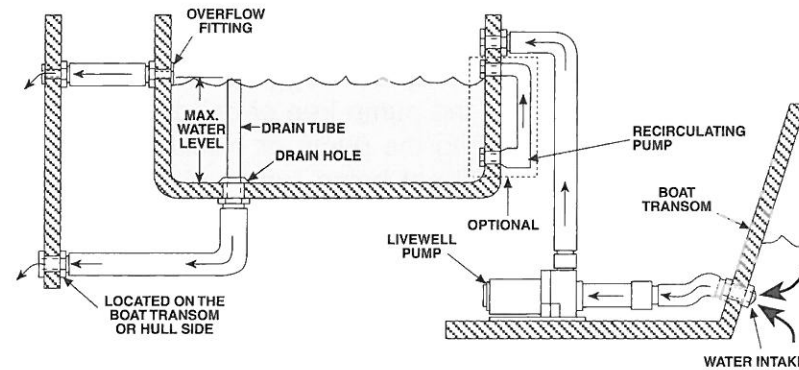
FIGURE 2.3 – MANUAL LIVEWELL
